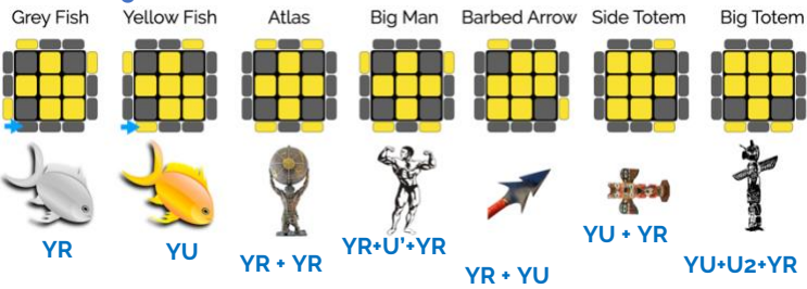
Algorithm 7
