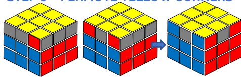
Algorithm 7
