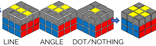
Algorithm 5
