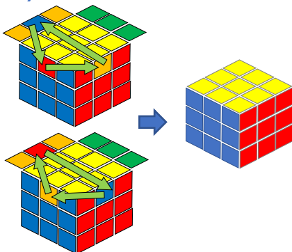
Algorithm 8
