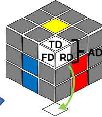
Bonus Algorithm 3
